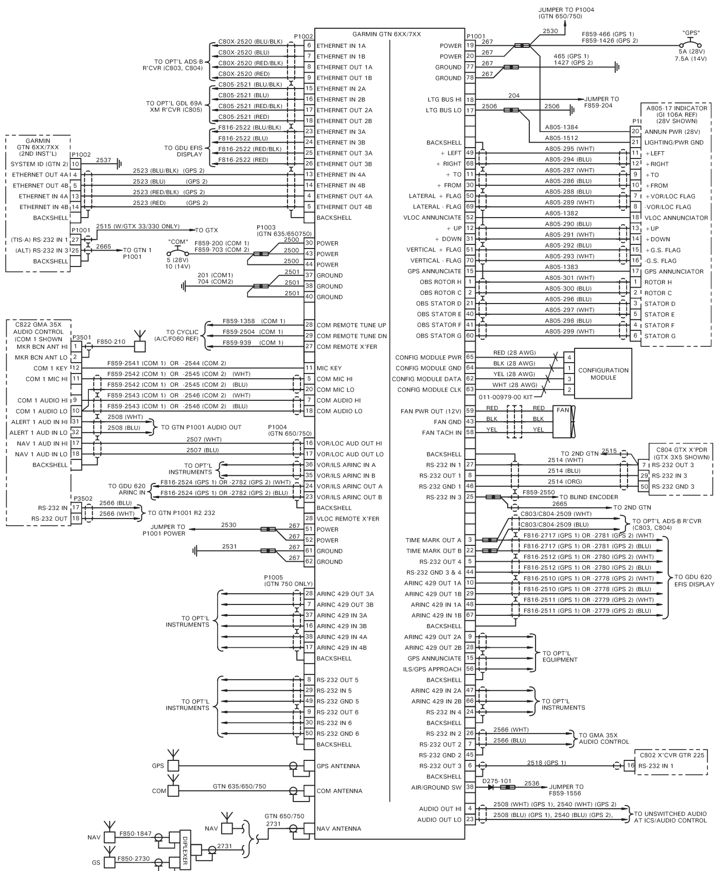
FIGURE 98-13 GARMIN GTN 6XX/7XX-SERIES GPS INSTALLATION (G500H EFIS)
