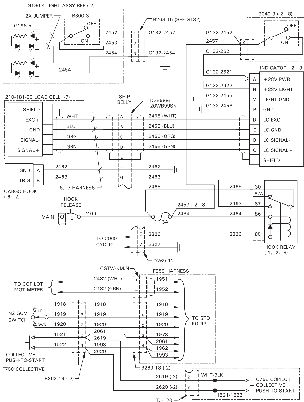
FIGURE 98-28 CARGO HOOK INSTALLATION
