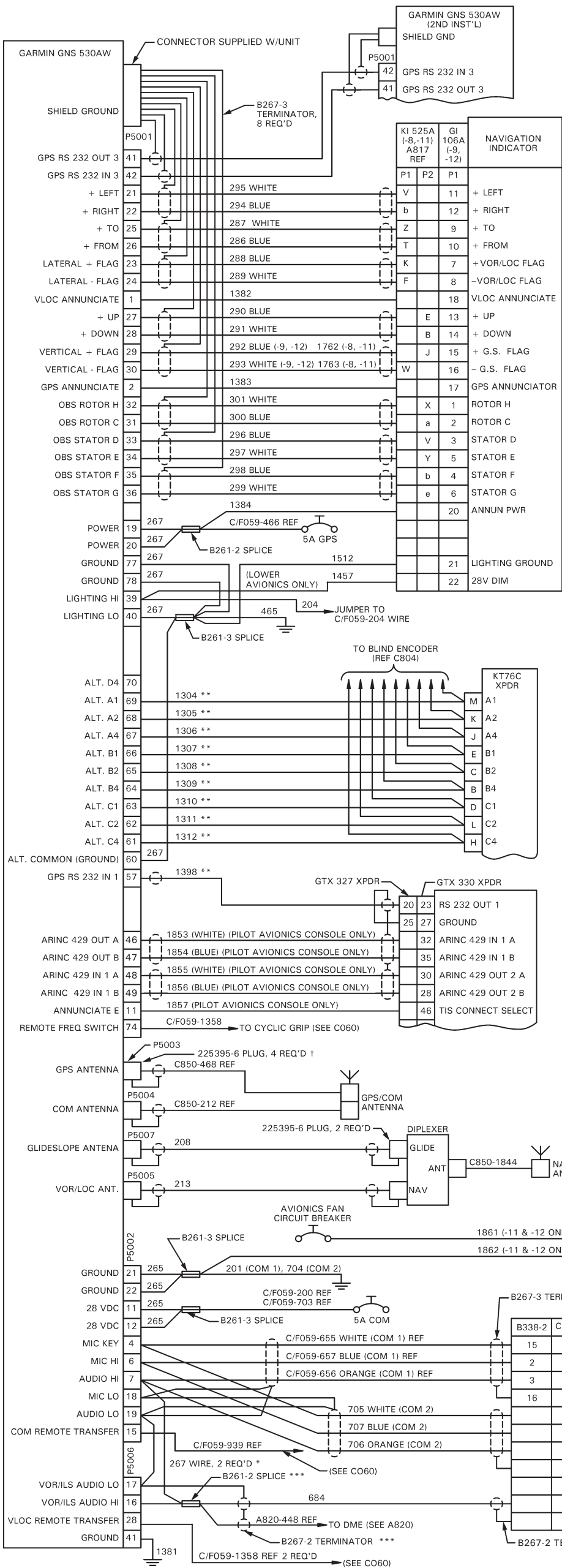
FIGURE 98-13C GARMIN 500 SERIES GPS INSTALLATION
