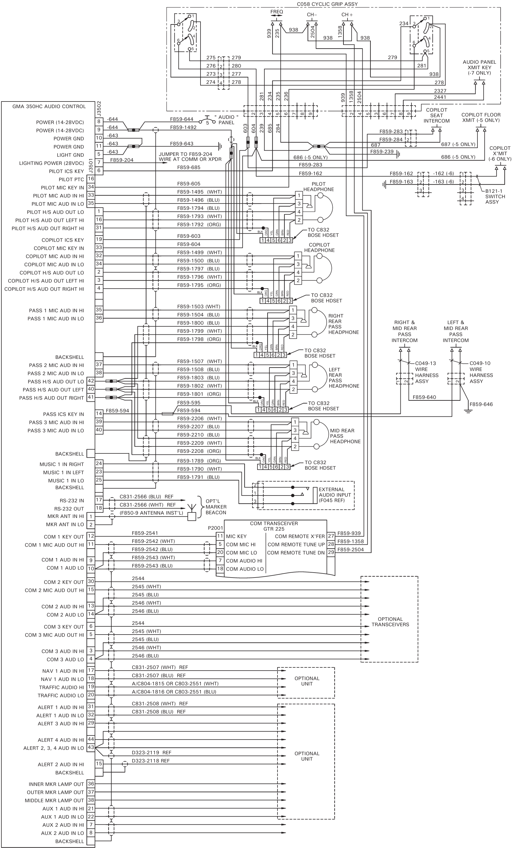
FIGURE 98-25A F060-4, -5, -6, & -7 INTERCOM SYSTEM INSTALLATION (GARMIN GMA 350HC AUDIO CONTROL)
