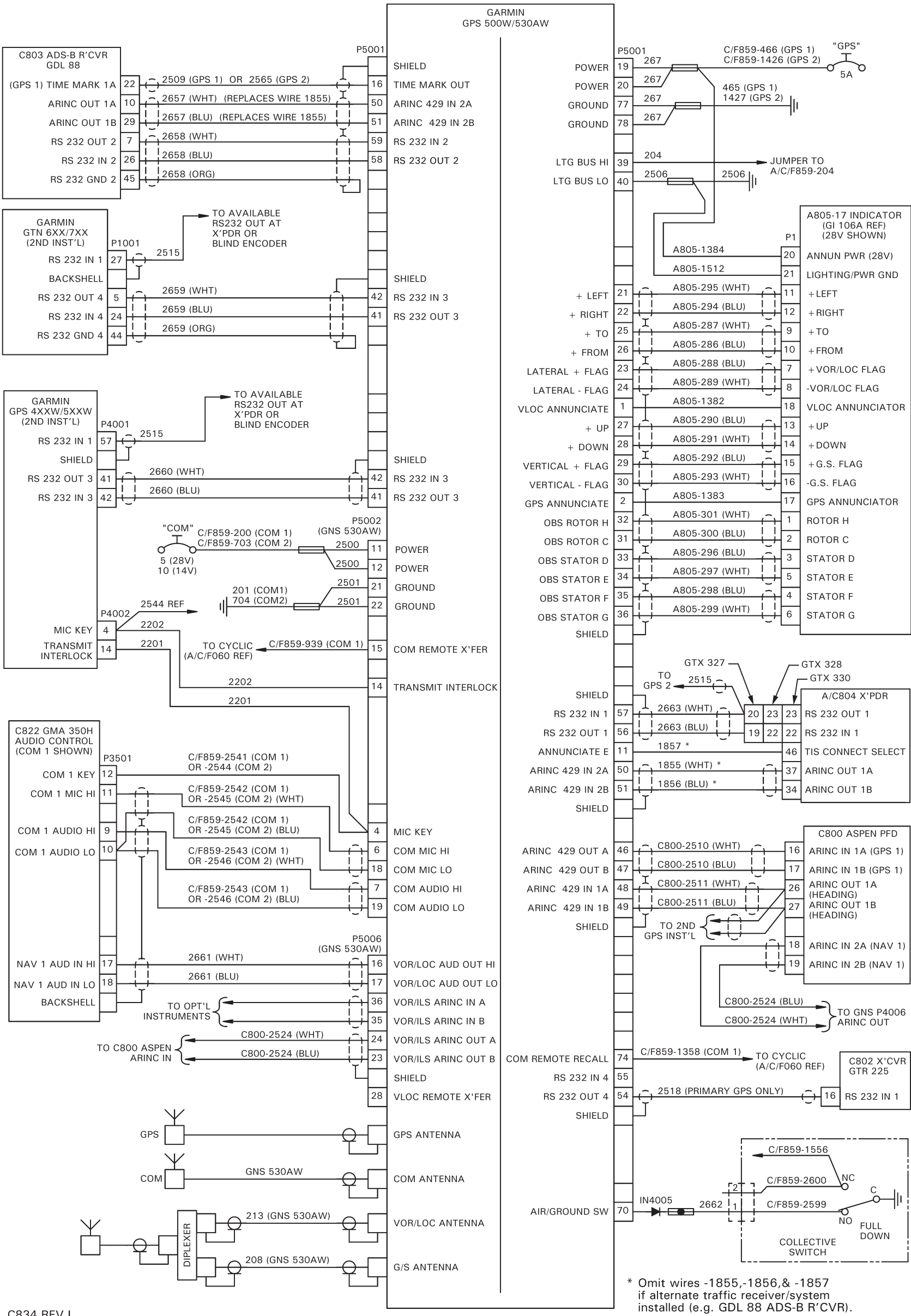
FIGURE 98-13B GARMIN 500 SERIES GPS INSTALLATION
