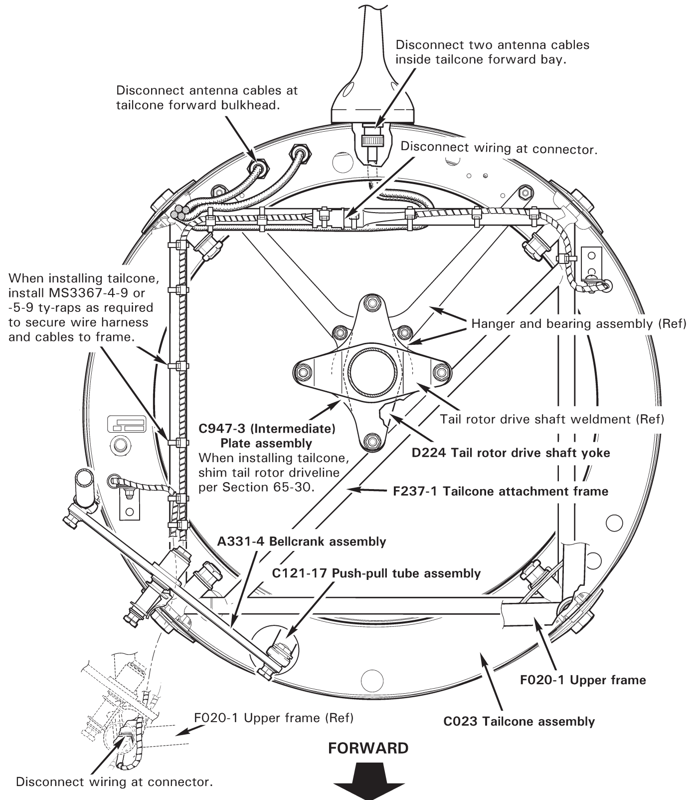
FIGURE 53-4 TAILCONE ASSEMBLY
