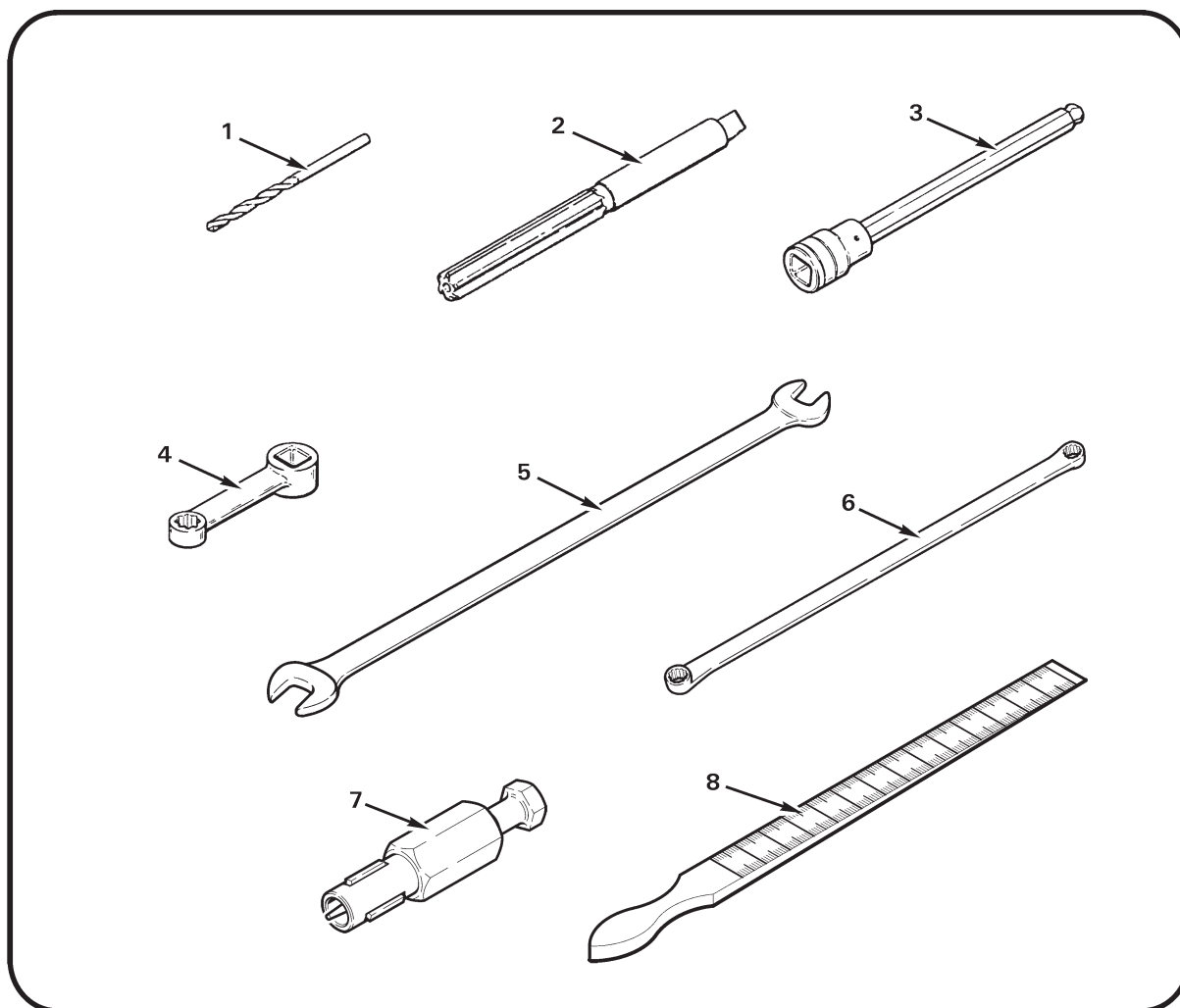
FIGURE 36-6 SPECIAL TOOLS
