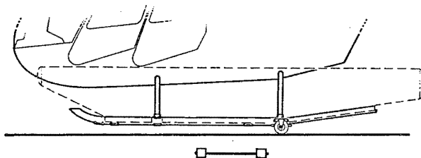
FIGURE 1-3B FLOAT SHIP GROUND HANDLING WHEELS INSTALLATION
